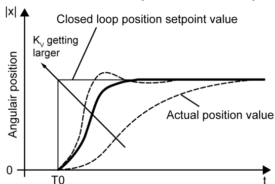
Transfer function of the position control loop, effect ID104 'Position loop factor KV'
