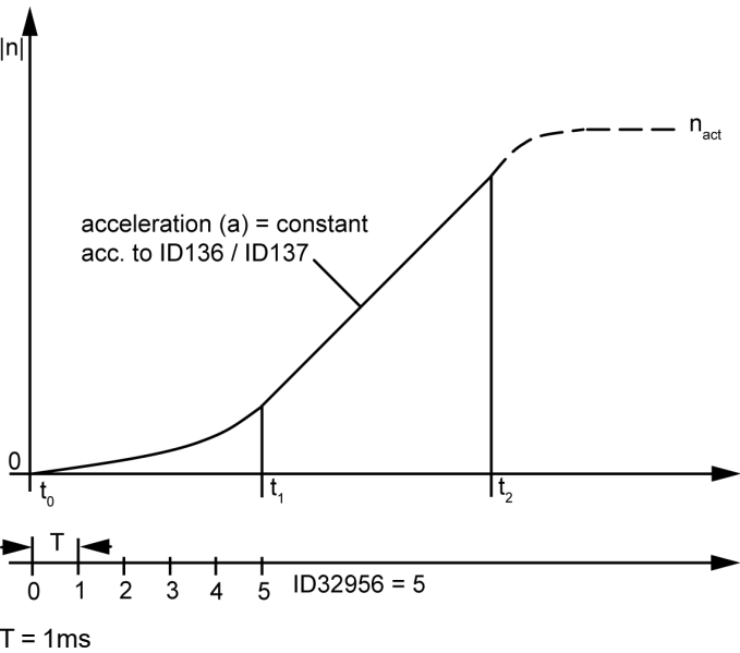
Velocity curve, acceleration coefficient
