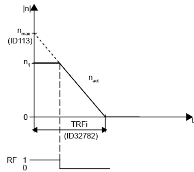
TRFi: Deceleration time RF inactive (ID32782)
